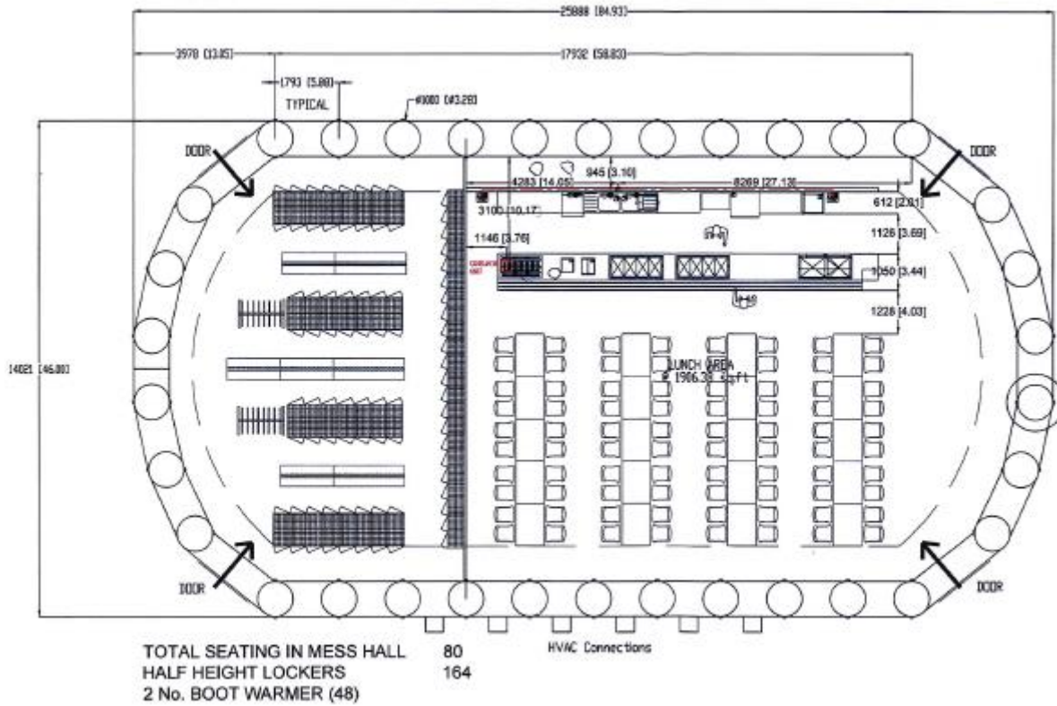
INDICATIVE FLOOR PLAN OF MESS / LOCKER SHELTER
